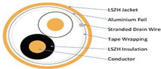
Shielded Cable
