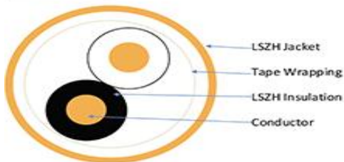
Shielded Cable
