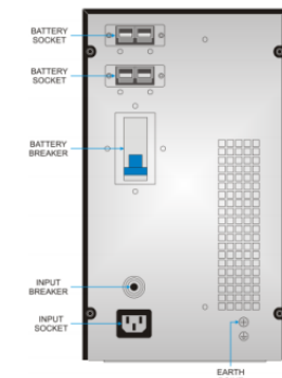
EE202 & EE203 Rear View
