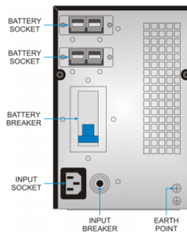
EE201 Rear View
