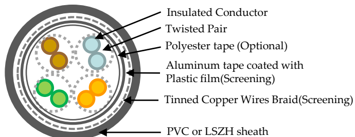
Fig 1. Cross Sectional Diagram of Cable
