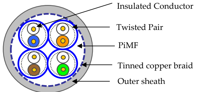
Fig 1. Cross Sectional Diagram of Cable
