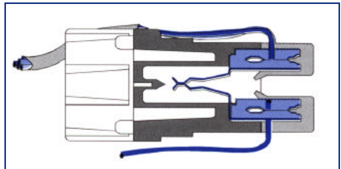
Highband Disconnect Contact
