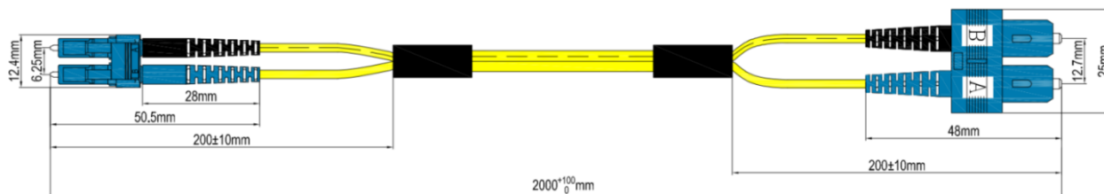
Dimensional drawing
